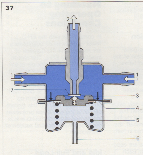
Fig. 37 Cross-sectional drawing of the fuel-pressure regulator
