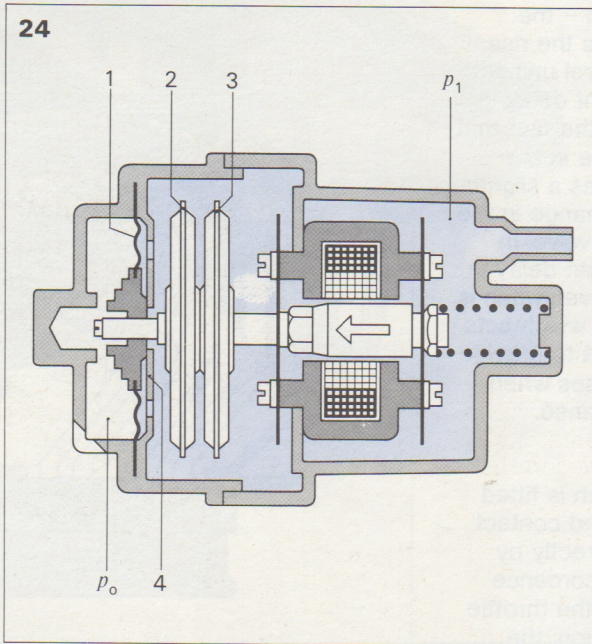
Fig. 24 Pressure sensor at part load, p_1 < p_0 Basic operation: diaphragm cells (2/3) pressed lightly together Auxiliary operation: diaphragm (1) pressed against part-load stop (4) 1 Diaphragm 2 Diaphragm cell 3 Diaphragm cell 4 Part-load stop p_0 Atmospheric pressure p_1 Intake manifold pressure
