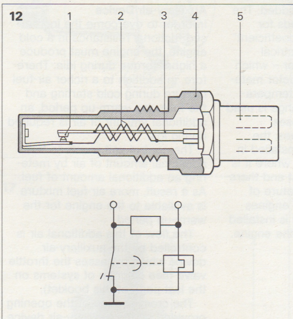
Fig. 12 Cross-sectional drawing of the thermo-time switch
