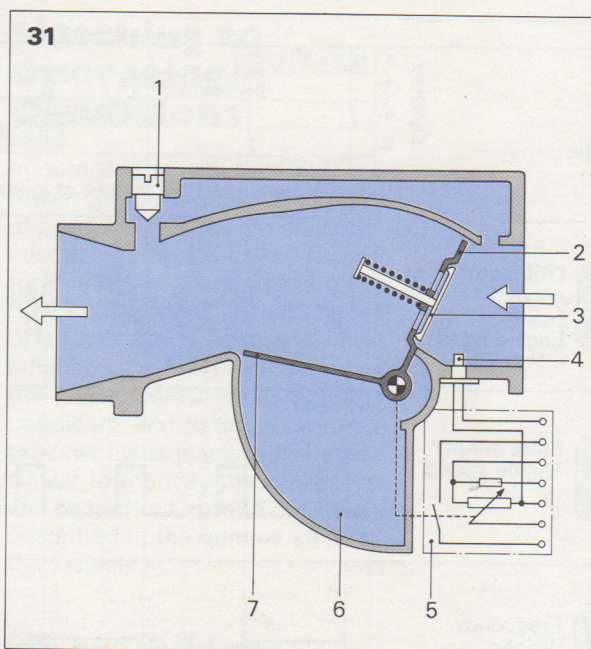
Fig. 31 Cross-sectional drawing of the air-flow sensor
