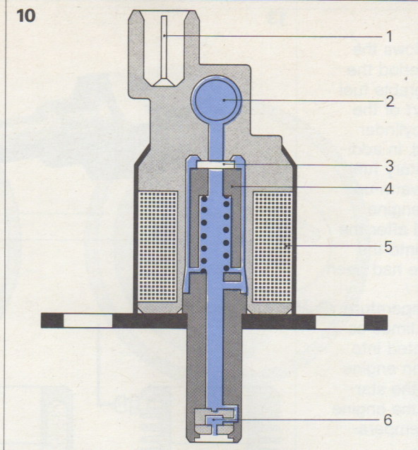
Fig. 10 Start valve
