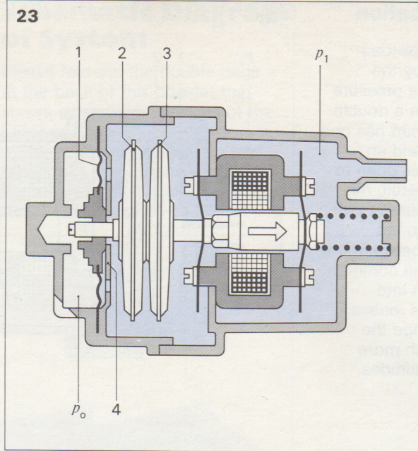
Fig. 23 Pressure sensor during idle, p_1 \ll p_0 Basic operation: diaphragm cells (2/3) expanded. Auxiliary operation: diaphragm (1) pressed against part-load stop (4) 1 Diaphragm 2 Diaphragm cell 3 Diaphragm cell 4 Part-load stop p_0 Atmospheric pressure p_1 Intake manifold pressure
