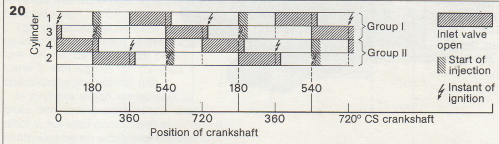
Fig. 20 Fuel injection timing diagram (EFI-D)
