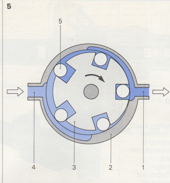
Fig. 5 Roller-cell pump 1 Pressure side 2 Pump housing 3 Pump rotor 4 Suction side 5 Roller
