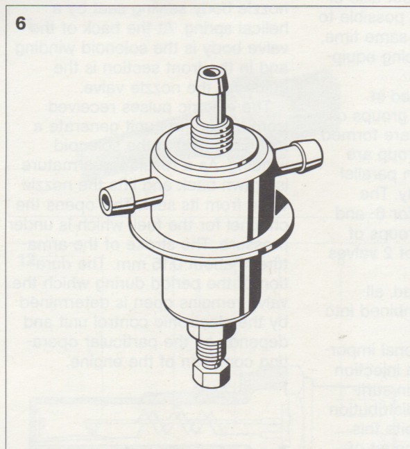
Fig. 6 Fuel-pressure regulator (EFI-D)
