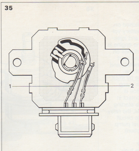
Fig. 35 Throttle valve switch
