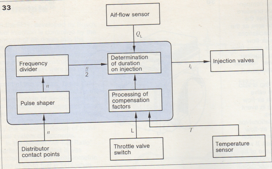
Fig. 33 Block operating diagram of the EFI-L Signals for: n Rotational speed Q_L Amount of air T Temperature t_i Duration of injection L Idle, full-load
