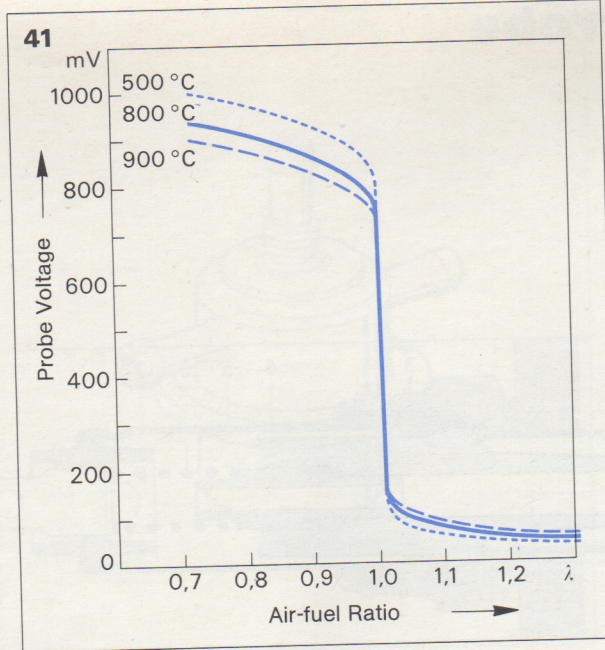
Fig. 41 Operating characteristic of the Lambda probe
