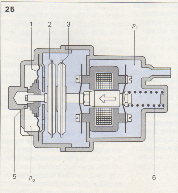
Fig. 25 Pressure sensor at full-load, p_1 \approx p_0 Basic operation: diaphragm cells (2/3) pressed together Auxiliary operation: diaphragm (1) pressed against full-load stop (5) 1 Diaphragm 2 Diaphragm cell 3 Diaphragm cell 5 Full-load stop 6 Spring p_0 Atmospheric pressure p_1 Intake manifold pressure
