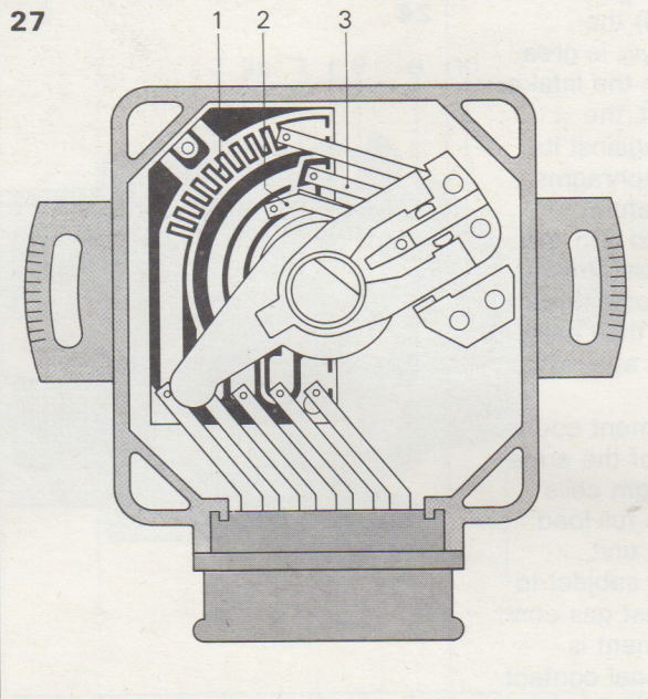
Fig. 27 Throttle valve switch
