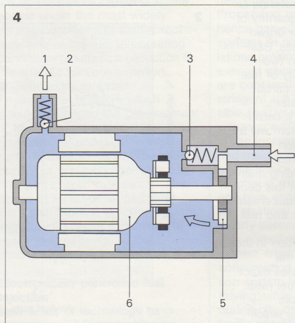
Fig. 4 Electric fuel pump
