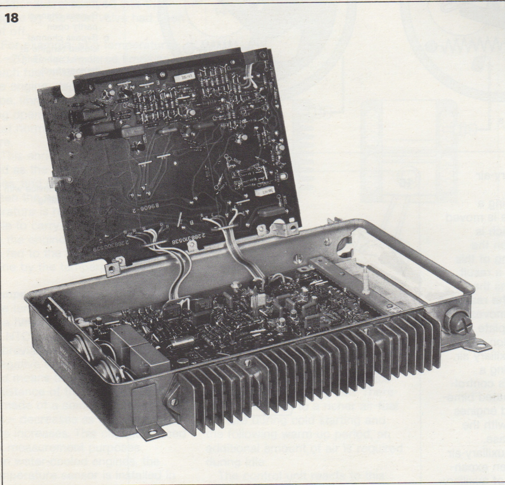
Fig. 18 Control unit in the EFI-D
