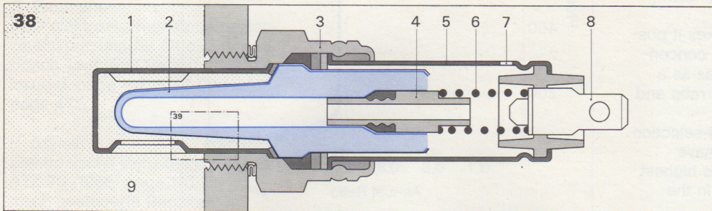
Fig. 38 Cross-sectional drawing of the Lambda probe
