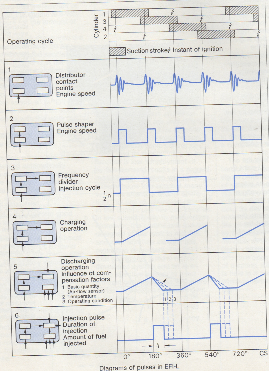
Fig. 34 Diagram of pulses in EFI-L
