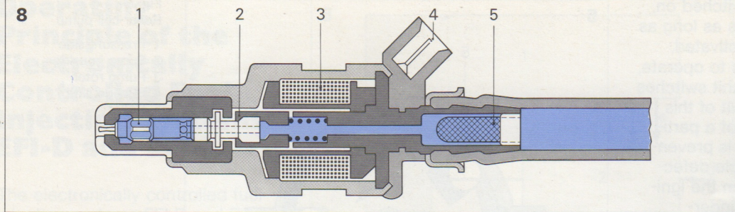
Fig. 8 Cross-sectional drawing of the injection valve
