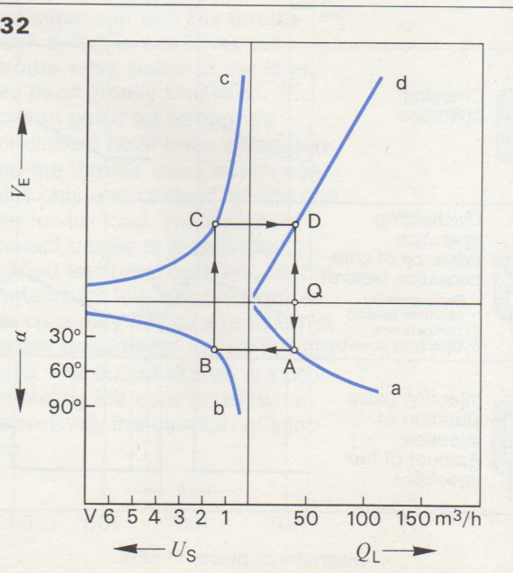
Fig. 32 Relationships between volume of air, sensor flap angle, potentiometer voltage, and amount of fuel injected
